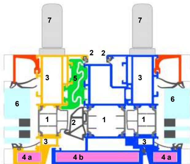
Horizontal section of a S6 energy saving French casement
